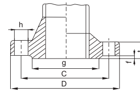
Standard dimensions of a 40Kgf/cm 2 Pipe flange
