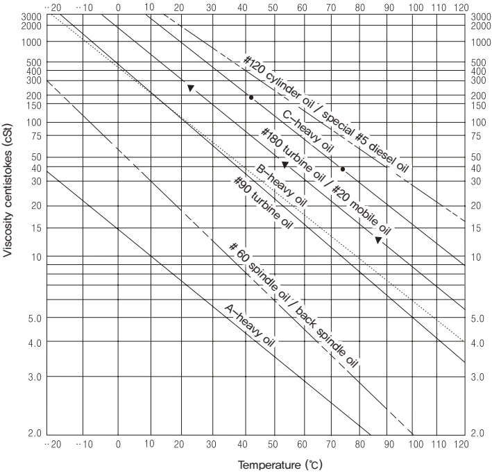
Oil temperature and viscosity curve
