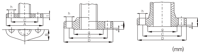
Standard dimensions of a 5kgf/cm 2 Pipe flange
