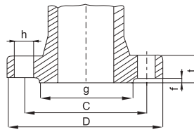
Standard dimensions of a 30Kgf/cm 2 Pipe flange
