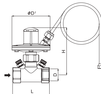
Differential pressure fixing type
