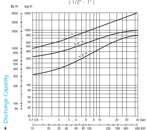
Discharge Capacities (1/2" - 1")
