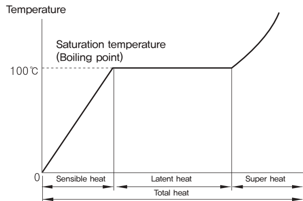
Diagram 2. Heat curve
