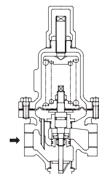
Pilot primary pressure regulating valve
