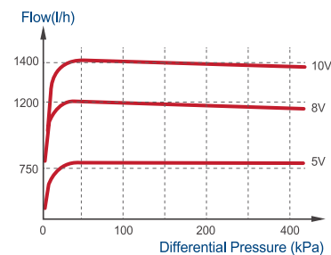
Pressure differential + Voltage control characteristics
