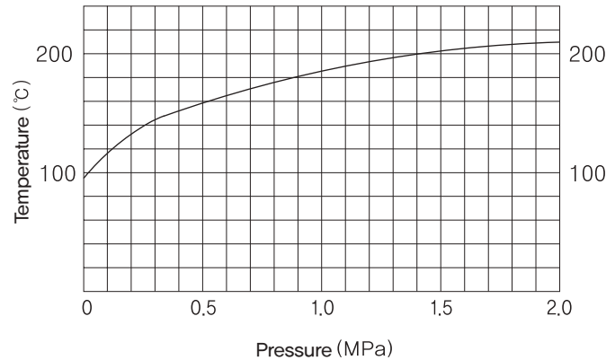
› Diagram 1. Steam curve
