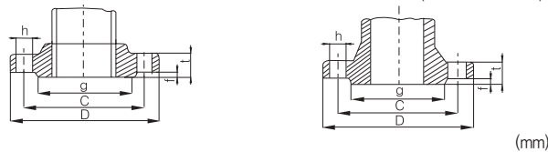
Standard dimensions of an ANSI 125 POUND cast Pipe flange
