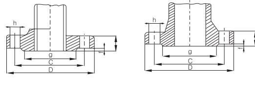
Standard dimensions of a 10kgf/cm 2 Pipe flange
