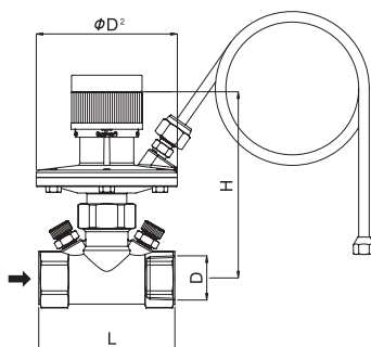
Differential pressure control type
