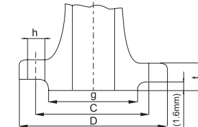
Standard dimensions of an ANSI 150 POUND cast Pipe flange
