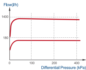
Pressure differential characteristics
