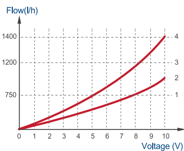
Voltage Control
