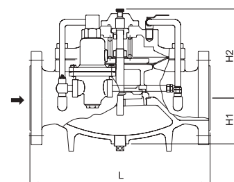
Main valve
