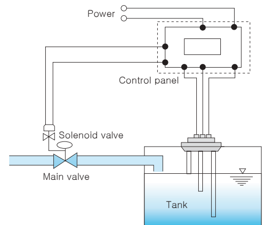
Diagram 2. Solenoid valve connecting circuit
