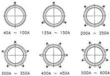
Packing Cylinder Orientation
