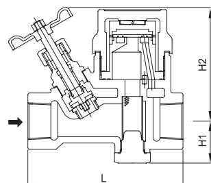
Type YSP-1 (Bypass valve attached)
