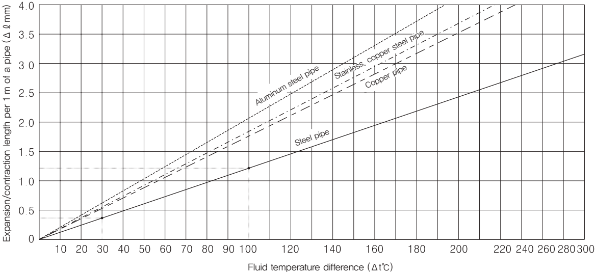
► Diagram 1 Expansion/contraction length of a pipe (Expansion/contraction length per 1 m of a pipe)
