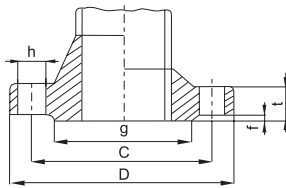
Standard dimensions of a 30Kgf/cm 2 Pipe flange
