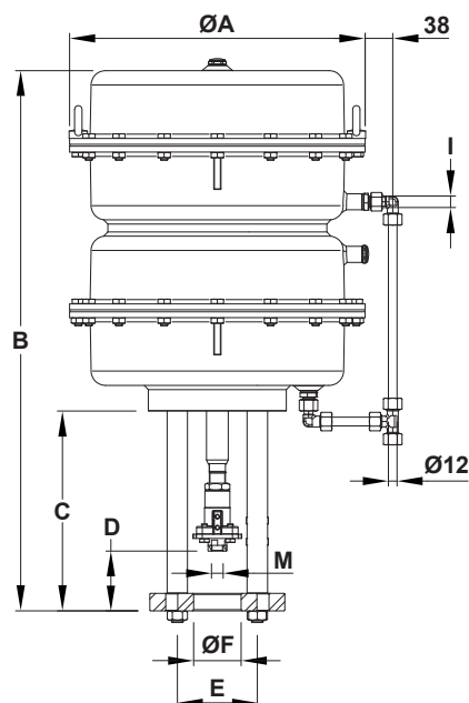
DIMENSIONS (mm)
