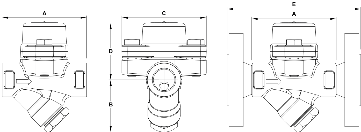
DIMENSIONS (mm)
